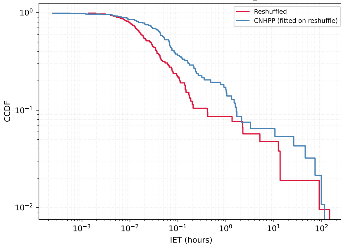
User 1065332141 - Reshuffled vs CNHPP A_{\text{fit}}=0.3724
